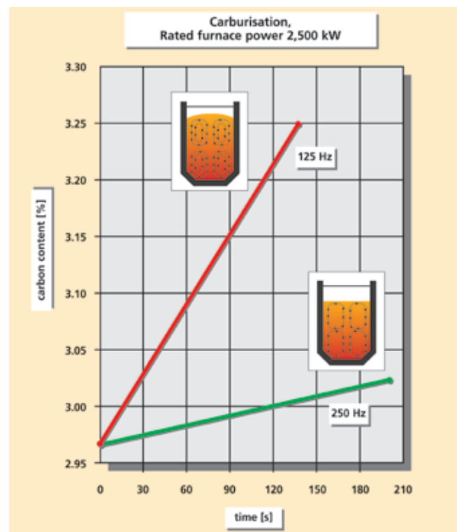
Multi-frequency technology
