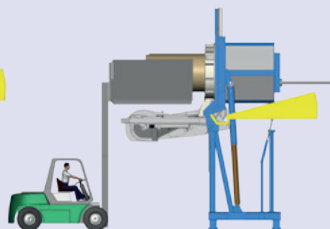
Easy crucible push-out without hood removal
