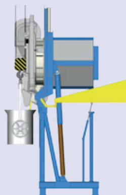
Narrow design for pouring into crane ladle
