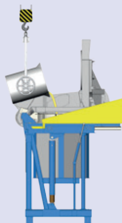
Easy backfilling
