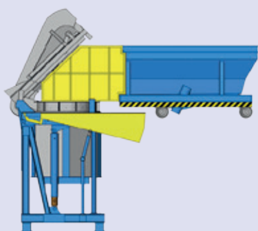
Optimum extraction during charging/melting
