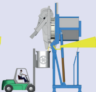
Optimum extraction during pouring into forklift ladle
