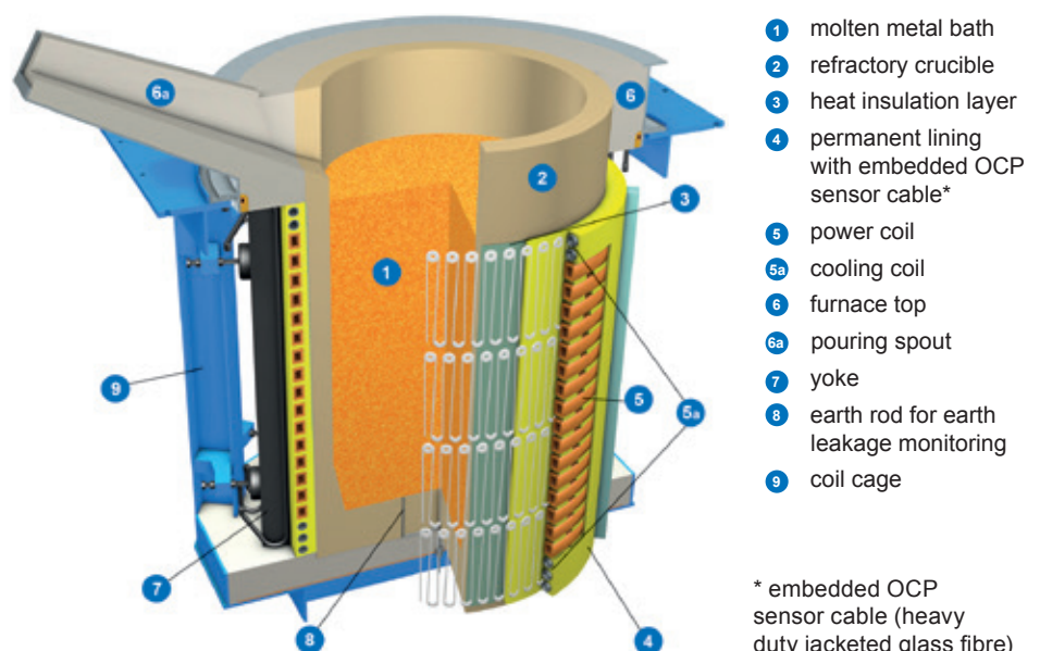
Coil assembly with OCP
